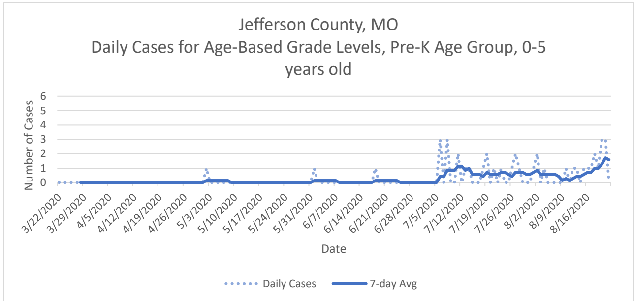
Figure 4. Daily Covid-19 Cases and 7-Day Rolling Average by Age-Based Grade Levels, Pre-K Age Group Jefferson County, Missouri
