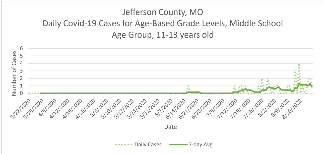
Figure 6. Daily Covid-19 Cases and 7-Day Rolling Average by Age-Based Grade Levels, Middle School Age Group Jefferson County, Missouri
